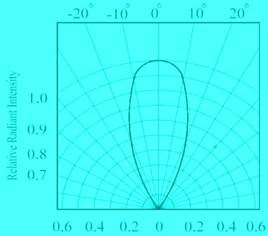
Fig.4 Relative Radiant Intensity vs. Angular Displacement
